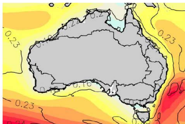
Business-as-usual scenario RCP8.5
